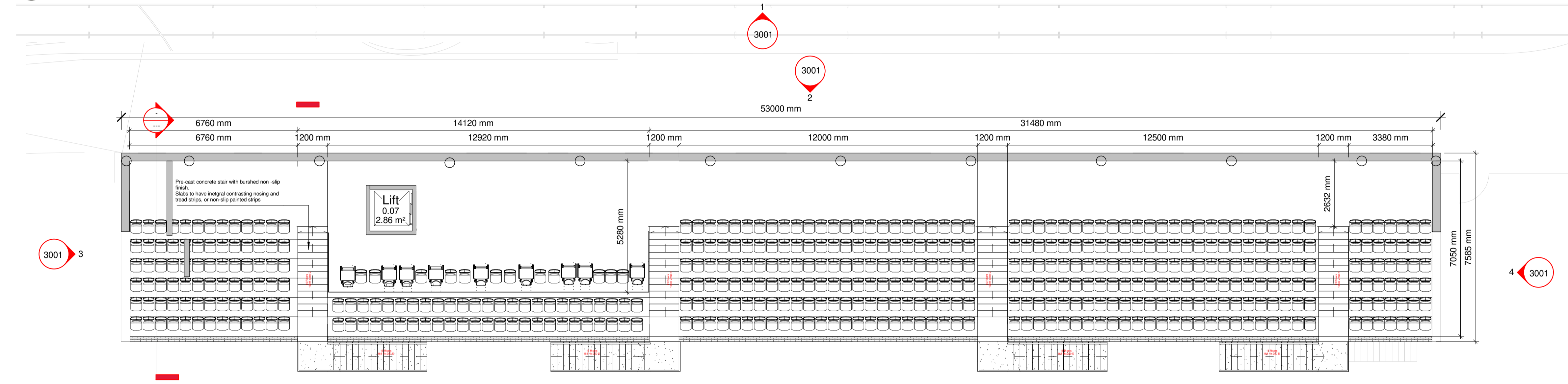
1 Plan - Ground Floor - GA 1 : 100
